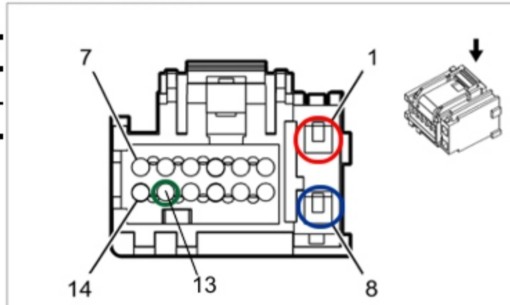
Fig 1: Radio X1 Connector End View
